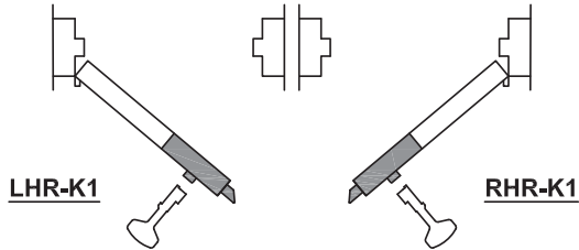
KEYED K1 HINGED SIDE HOLLOW METAL MOUNTING PLATE (FOR OUT-SWING DOORS)
