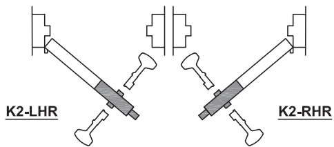
KEYED K2 HOLLOW METAL MOUNTING PLATE 1/2" BOLT PROJECTION (FOR OUT-SWING DOORS)
