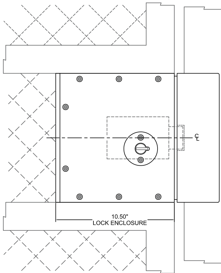
WLS-1780-K1 LHR GATE LOCK (SHOWN HINGE SIDE)
