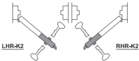
KEYED K2 HOLLOW METAL MOUNTING PLATE (FOR OUT-SWING DOORS)
