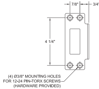
SS - STRIKE PLATE W/ INDICATION SWITCH
