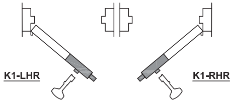
KEYED K1 HINGED SIDE HOLLOW METAL MOUNTING PLATE 1/2" BOLT PROJECTION (FOR OUT-SWING DOORS)
